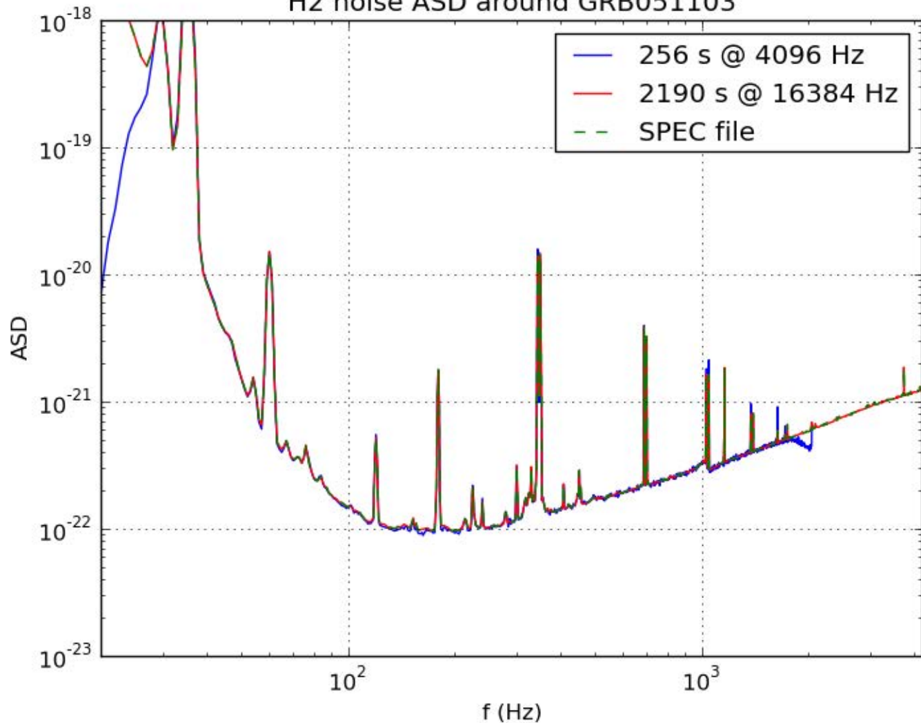
H2 noise ASD around GRB051103
