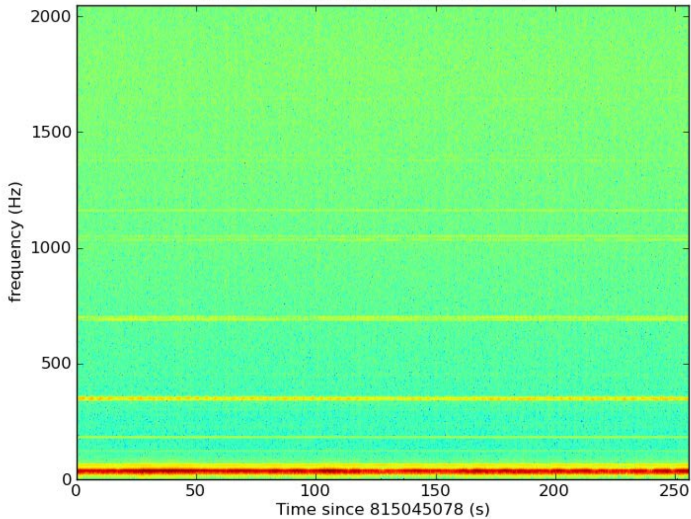
H2 spectrogram around GRB051103
