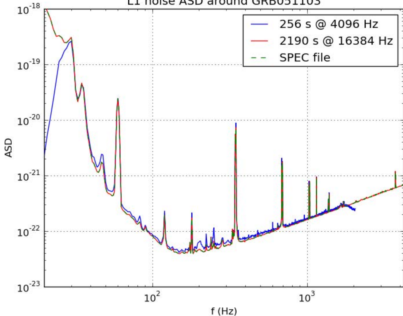
L1 noise ASD around GRB051103
