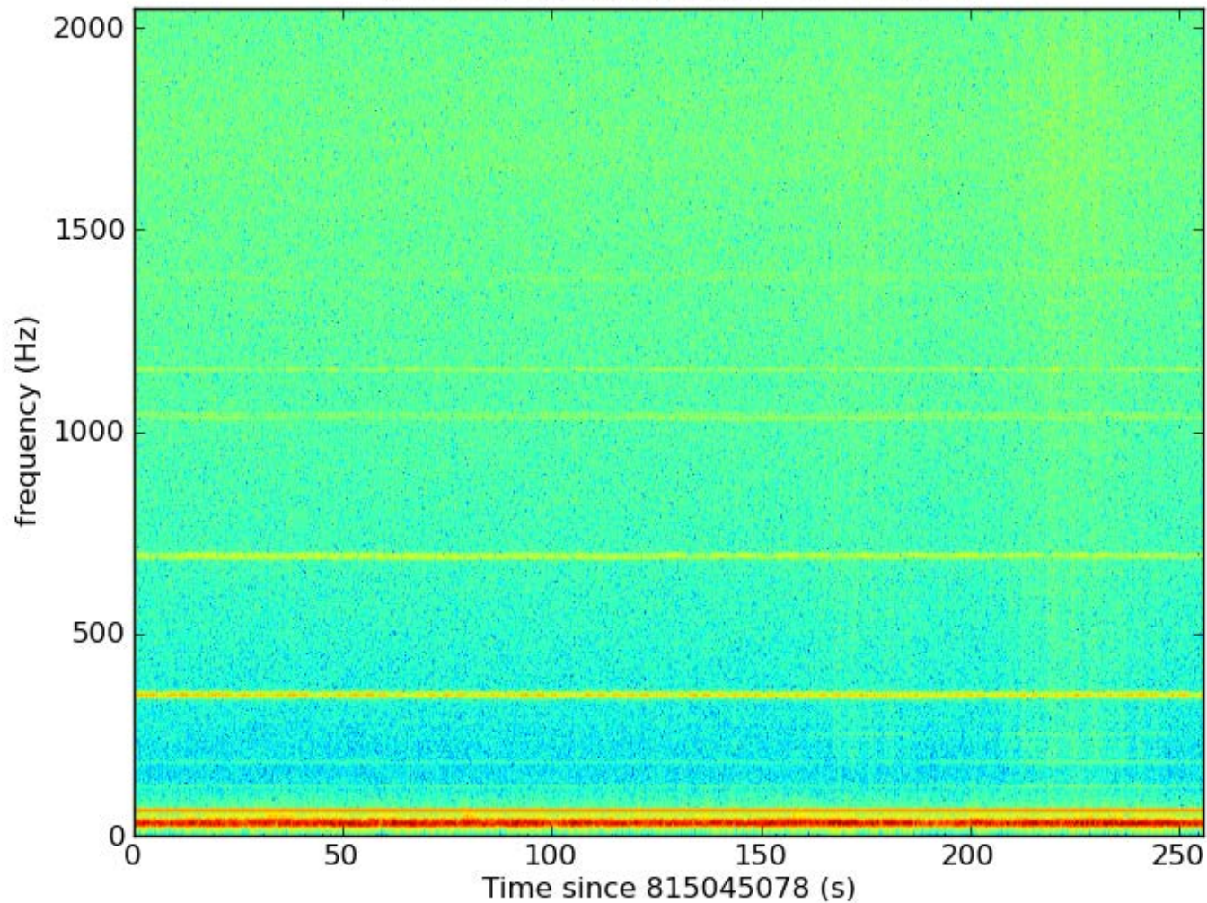
L1 spectrogram around GRB051103
